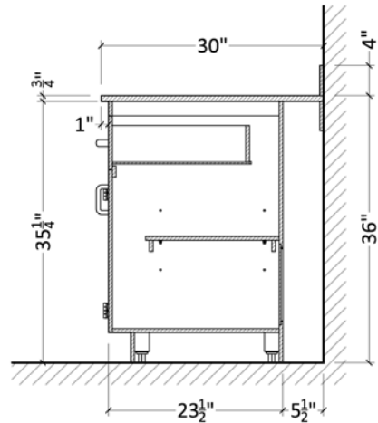
TYPICAL CABINET SECTION
