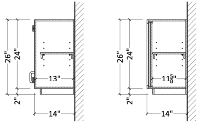
TYPICAL CABINET SECTIONS
